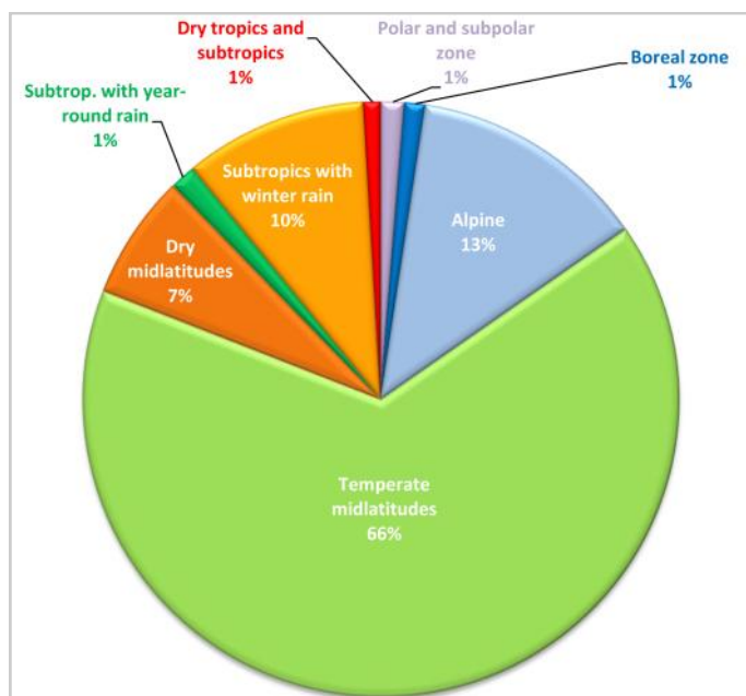
Fig. 5. Distribution of independent plots contained in GrassPlot v. 2.00 ( N = 28,171 ) across biomes as defined by Bruehlheide et al. (2019).
